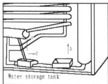
Water tank
