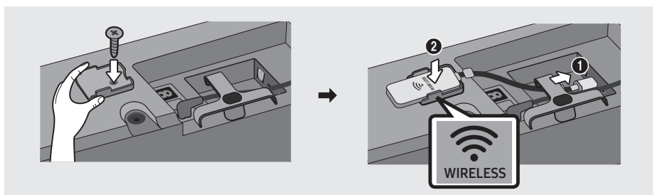
Fixation murale
