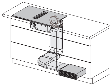
KMDA7272-1FL, KMDA7272FL, KMDA7473FL, KMDA7473-1FL – flush
