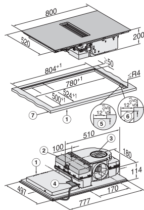
KMDA7272-1FL, KMDA7272FL, KMDA7473FL, KMDA7473-1FL – flush
