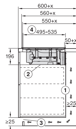
KMDA7272-1FL, KMDA7473-1FL/FL MattFinish, KMDA7272FL, KMDA7473FL – Side view lying on top+X, Plug&Play
