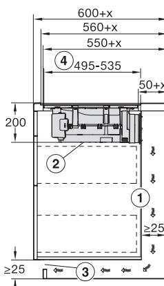
KMDA7272-1FL, KMDA7473-1FL/FL MattFinish, KMDA7272FL, KMDA7473FL – Side view flush+X, Plug&Play
