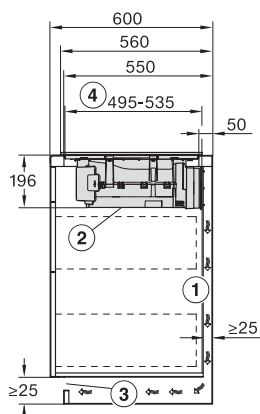
KMDA7272-1FL, KMDA7473-1FL/FL MattFinish, KMDA7272FL, KMDA7473FL – Side view lying on top, Plug&Play
